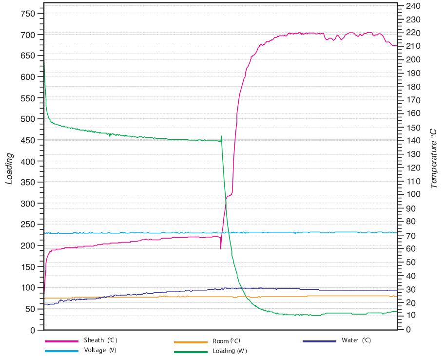
Performance in water-air @ 230V
